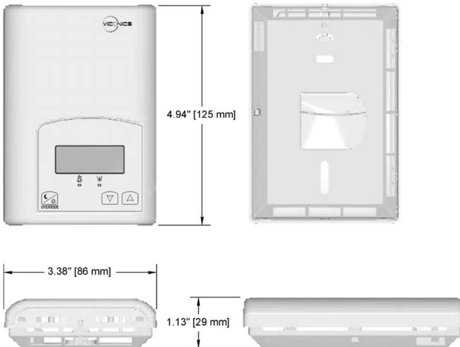
Fig.1 – Thermostat dimensions
